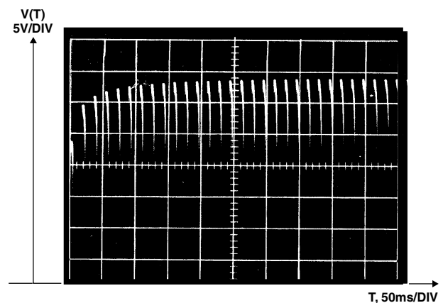
FIGURE 4. V130LA10A) VARISTOR VOLTAGE FOR THE INITIAL CYCLES OF 60Hz OPERATION AT A PEAK CURRENT OF 1.0mA
