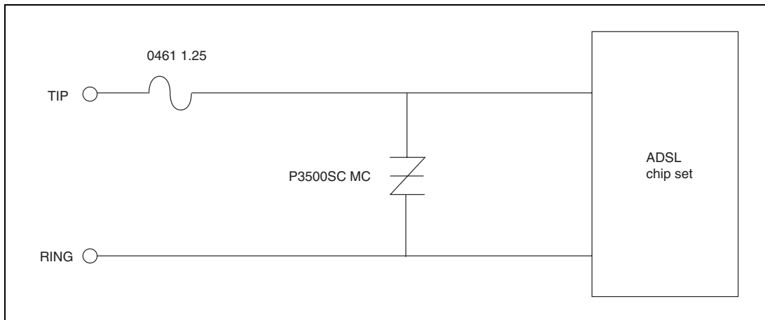
Figure 3.8 ADSL Protection
