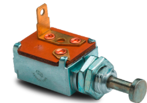
91812 12V 5A Normally Closed Self Grounded Door Switch
