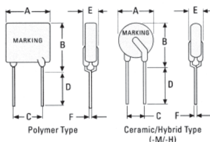
Dimensions (mm)
