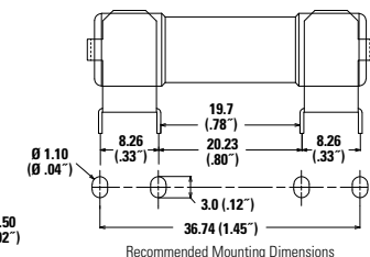
106 001 Device Dimensions
