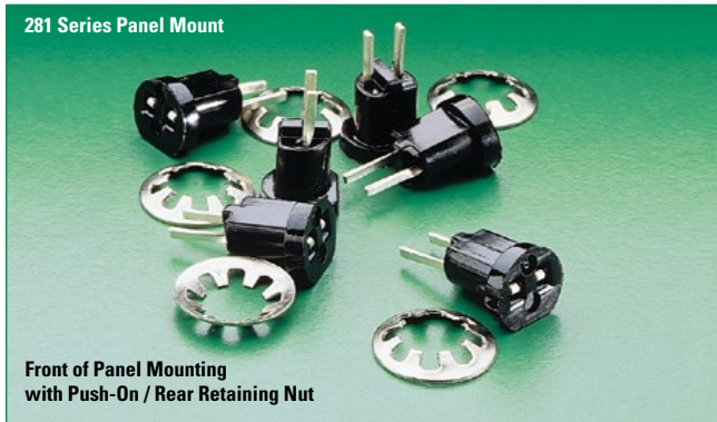
0281 0001 Front of Panel Mounting with Push-On / Rear Retaining Nut
