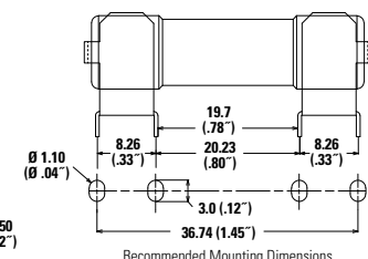
106 001 Device Dimensions
