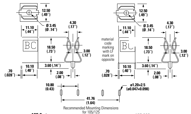
105 003 Device Dimensions
