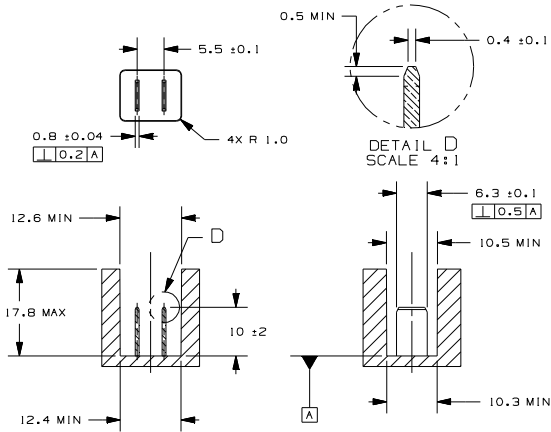
RECOMMENDED MATING CAVITY SCALE 1:1
