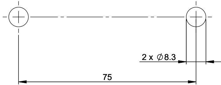
Mounting template
