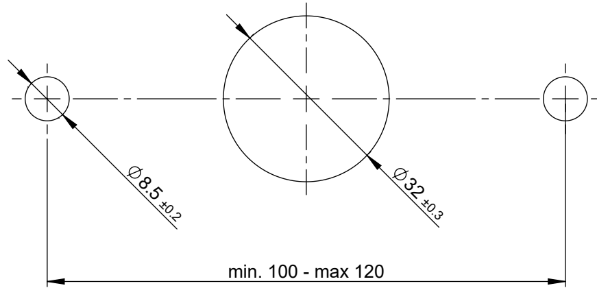
Fixing holes
