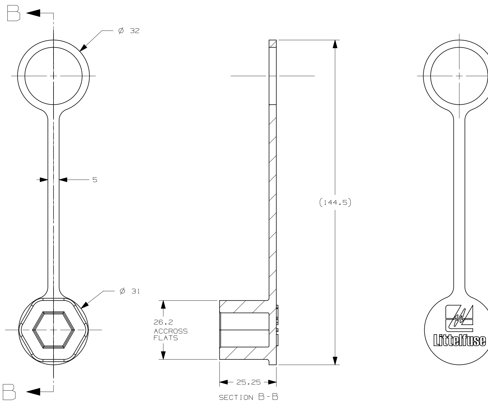
FIGURE 2. 3/8" STUD CAP
