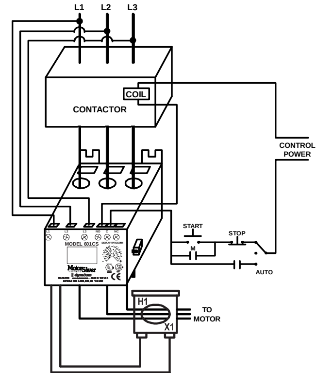
Figure 1: Typical Wiring Diagram for FLA of 1-175A
