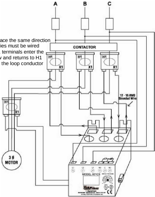
Figure 2: Typical Wiring Diagram Using External CTs.
