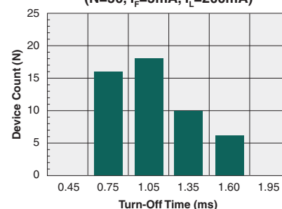
Typical Turn-Off Time (N=50, I_F=5\text{mA} , I_L=200\text{mA} )
