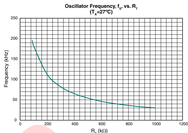
Figure 4 Resistor Selection
