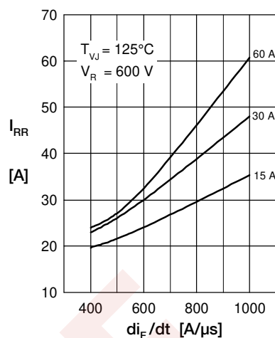
Fig. 3 Typ. peak reverse current I_{RM} versus di/dt
