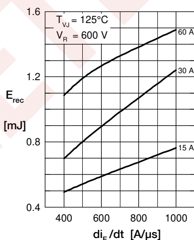
Fig. 6 Typ. recovery energy E_{rec} versus di/dt
