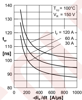
Fig. 5 Recovery time t_{rr} versus -di_F/dt
