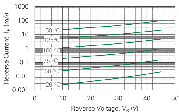
Figure 2. Typical Reverse Current vs. Reverse Voltage
