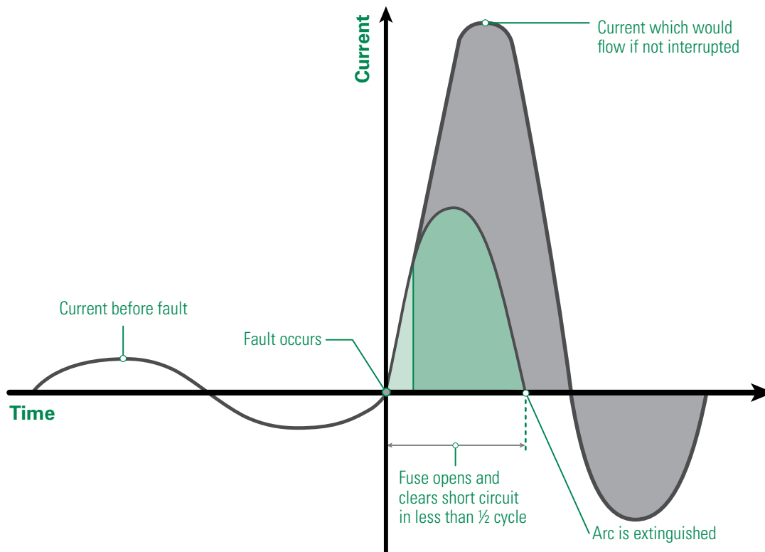
Figure 6: Current Limitation with a Current-Limiting Fuse (Source: Littelfuse)
