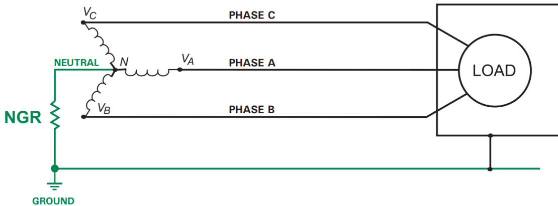
Figure 12: Resistance-Grounded Transformer
