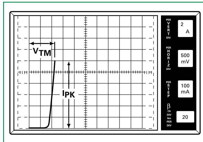
Figure AN1006.7 V_{TM} = 1.15 V at I_{T(peak)} = 12 A
