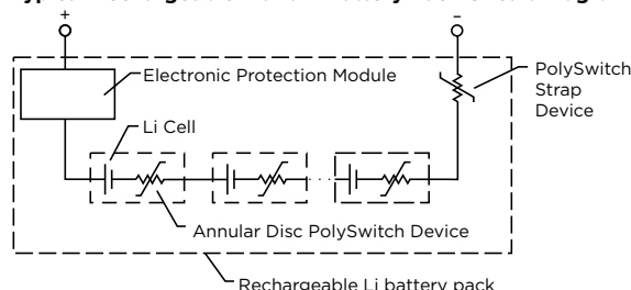
Typical Rechargeable Lithium Battery Pack Circuit Diagram
