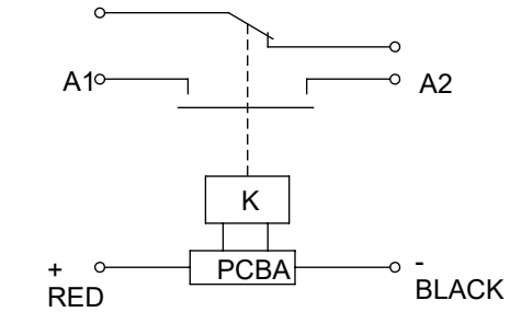
DCNHE250UF SERIES SCHEMATIC CIRCUIT DIAGRAM
