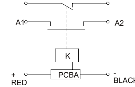
DCNHE250MF SERIES SCHEMATIC CIRCUIT DIAGRAM
