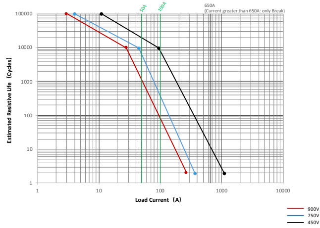
DCNHR50 / DCNHR100
