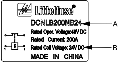
NAME PLATE
