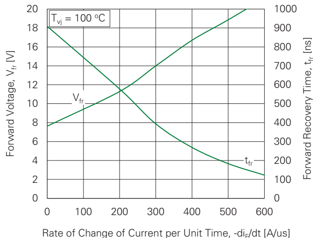
Fig. 5. Typical Forward Voltage V_{fr} and t_{fr} vs -di_F/dt
