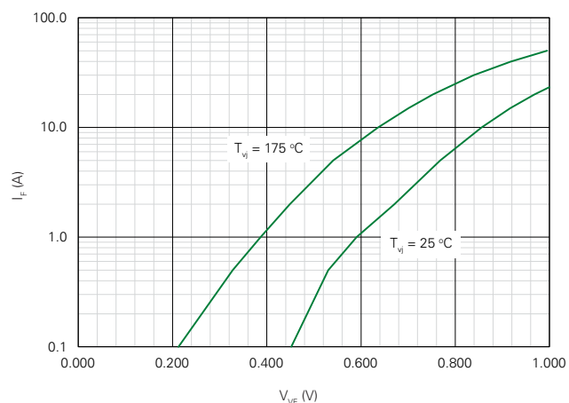
Fig. 1. On-State Current vs. On-State Voltage (Typical)
