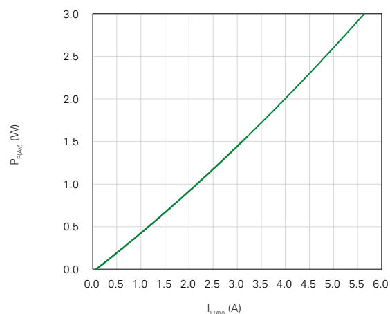
Fig. 2. Power Dissipation vs. Average Forward On-State Current (Typical)
