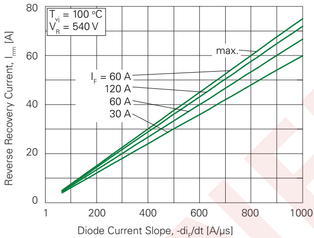
Fig. 3. Typical Peak Reverse Recovery Current vs. Diode Current Slope
