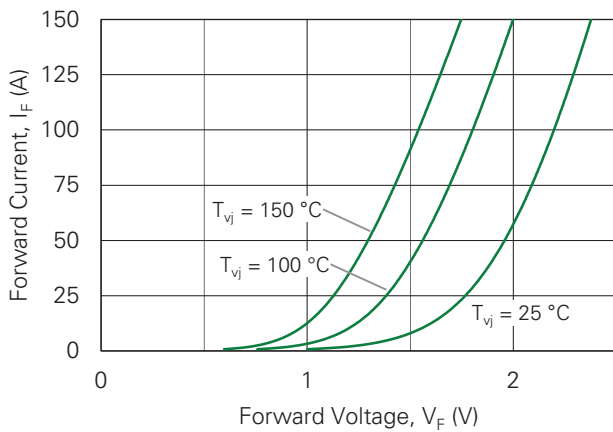
Figure 1. Forward Characteristics
