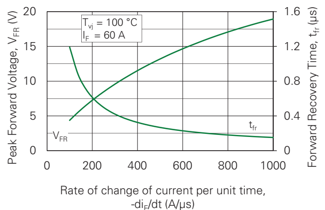
Figure 6. Typical Peak Forward Voltage V_{FR} and t_{fr} vs. -di_F/dt
