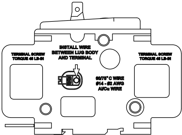
1/4" QUICK CONNECT (4)
