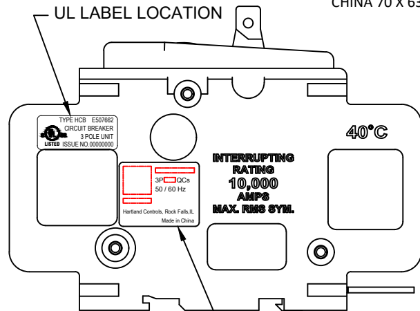
INDIVIDUAL BOX LABEL #1 - 1006397 (2.00"[50.80] x 2.19"[55.63]) CHINA 70 X 63
