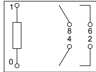
SCHEMATIC TERMINAL LOCATION COIL VOLTAGE 24 VAC 50/60 Hz
