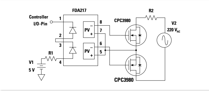
FDA217 used with CPC3980 MOSFETs to create Normally Closed Solid-state Relay
