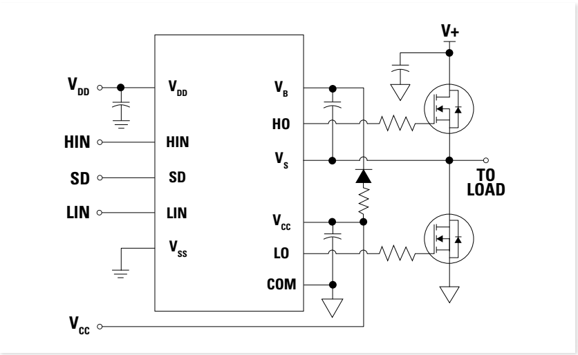
LF2110 and LF2113 Application Circuit
