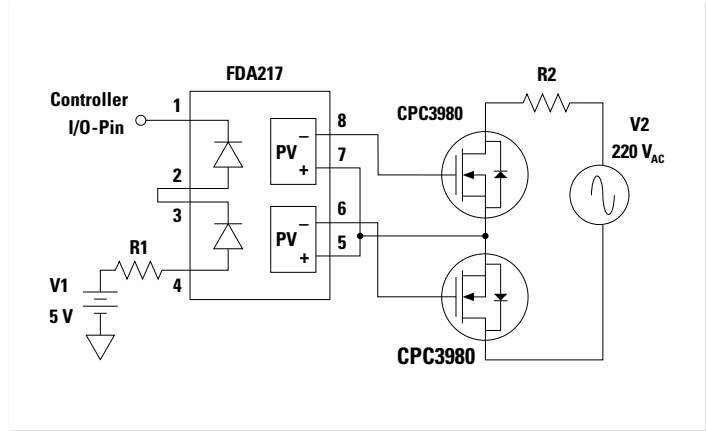
FDA217 used with CPC3980 MOSFETs to create Normally Closed Solid-state Relay
