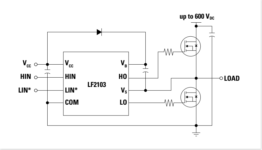
LF2103 Application Circuit
