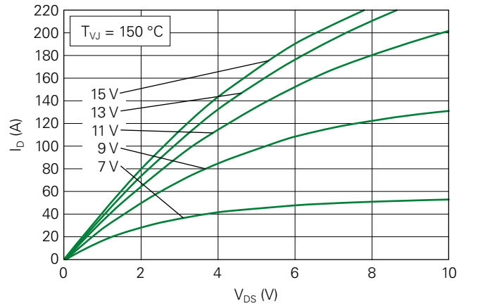
Fig. 6. Typical Output Characteristics ( T_{VJ} = 150 °C)
