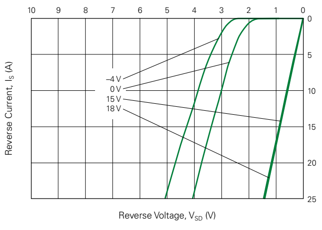
Fig. 11. Typical Reverse Conduction Characteristics @ T_{vj} = 25\text{ °C}
