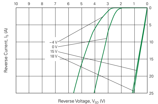
Fig. 10. Typical Reverse Conduction Characteristics @ T_{vj} = -40\text{ °C}
