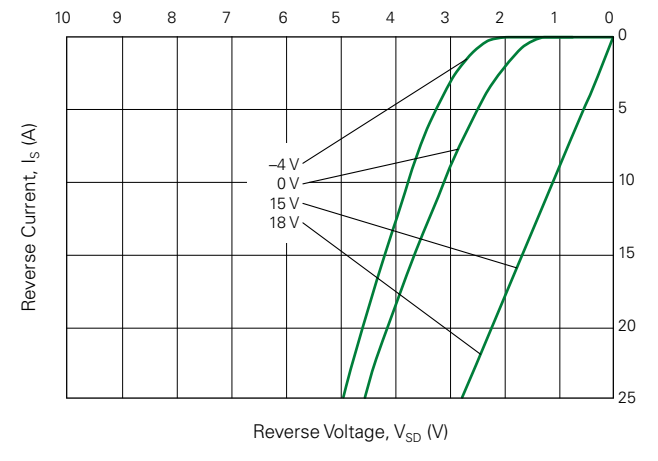
Fig. 12. Typical Reverse Conduction Characteristics @ T_{vj} = 150\text{ °C}
