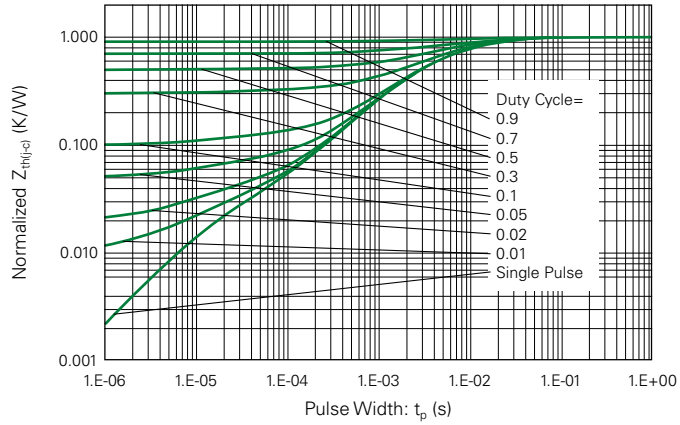
Fig. 25. Thermal Impedance (Normalized)
