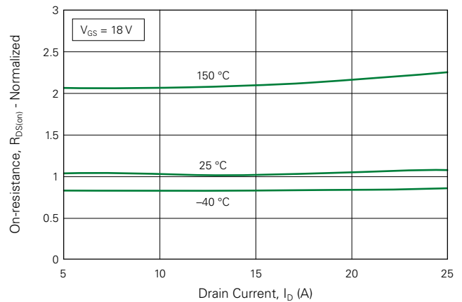
Fig. 6. R_{DS(on)} Normalized to I_D = 12 A vs. Drain Current
