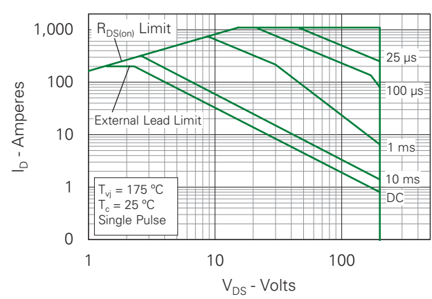
Fig. 14. Forward-Bias Safe Operating Area
