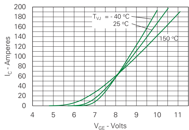
Fig. 6. Input Admittance
