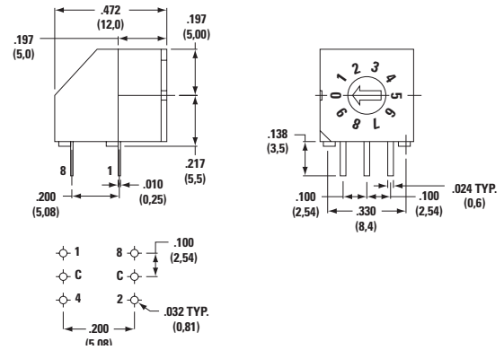
A Right Angle, PC Thru-hole
