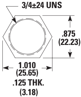
N With Nut Nut part number: 937C00000
