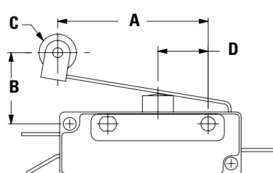
Figure 8 Leaf Roller
