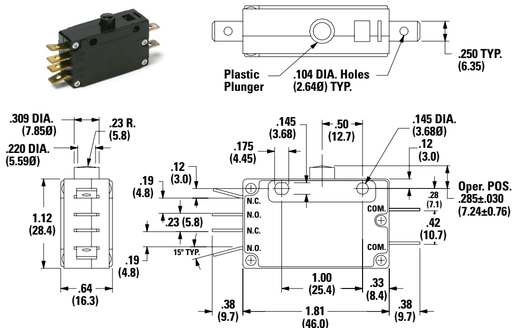
D Double Pole Switch Dimensions inches (mm)
