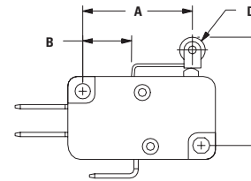
Figure 1, Lever Roller
