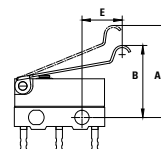
R05 Hinged Simulated Leaf Roller 5.0 mm
