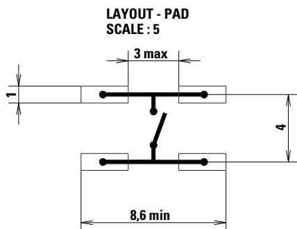
Pad Layout for J Versions
