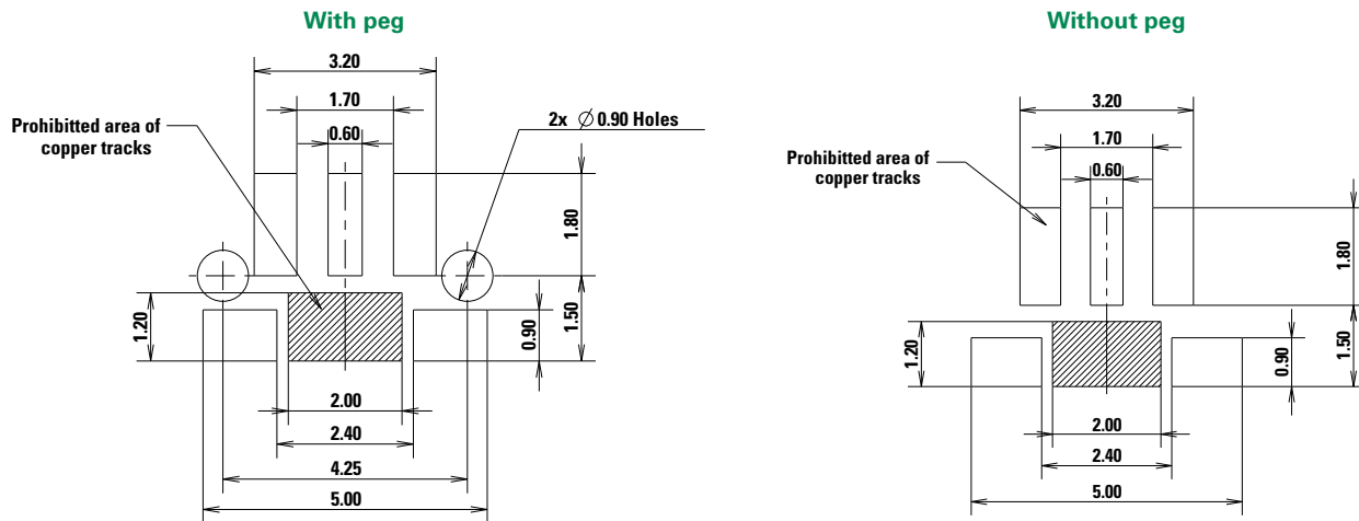
Pad Layout Dimensions (mm)
