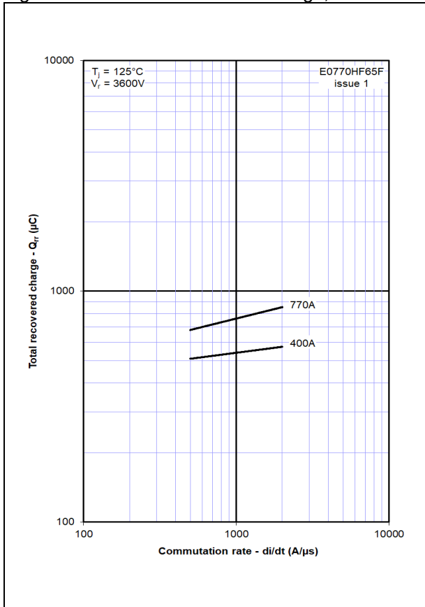
Figure 3 – Maximum recovered charge, Q rr
