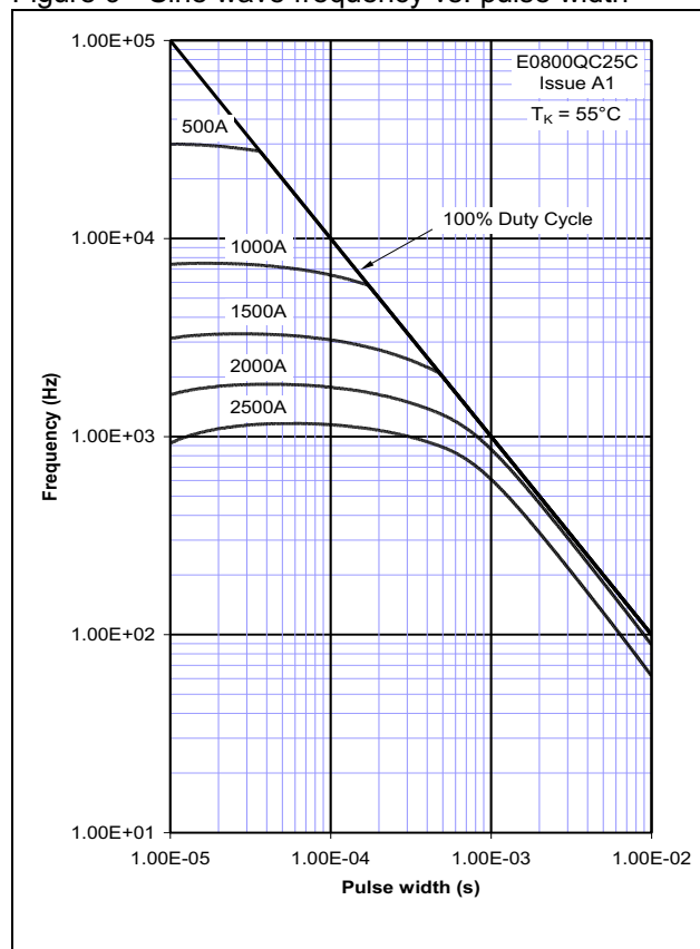
Figure 9 - Sine wave frequency vs. pulse width
