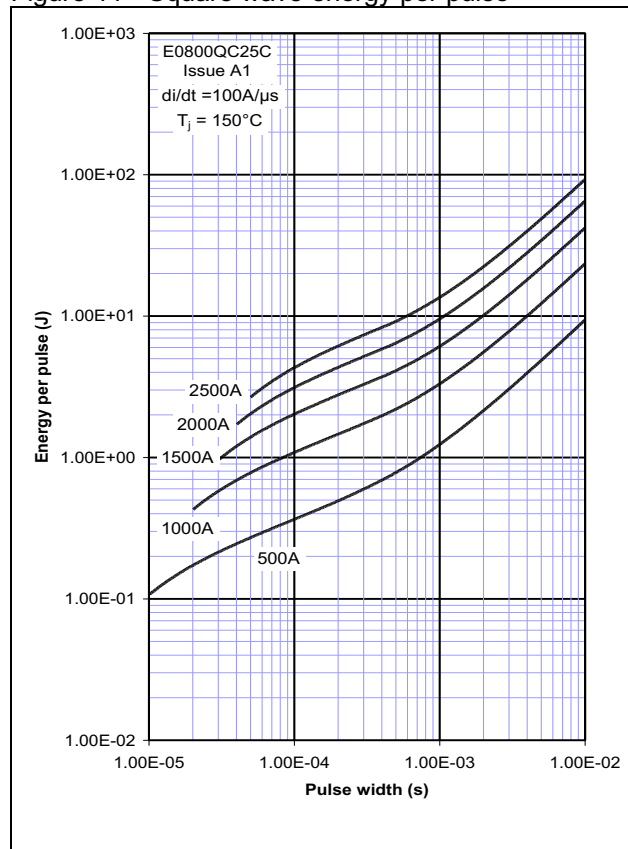
Figure 11 - Square wave energy per pulse
