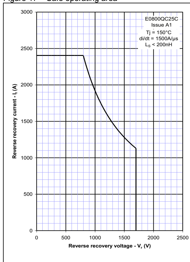
Figure 17 – Safe operating area
