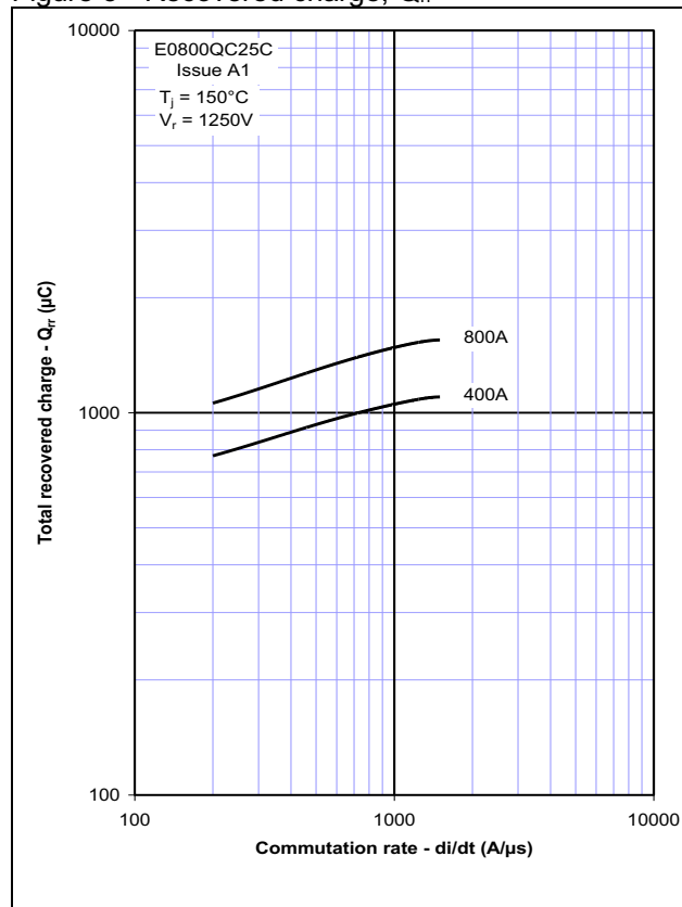
Figure 3 - Recovered charge, Q_{rr}
