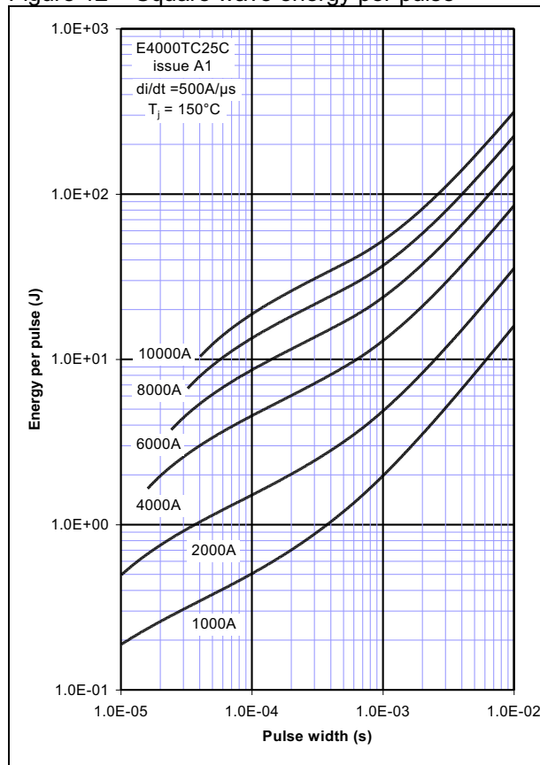
Figure 12 - Square wave energy per pulse
