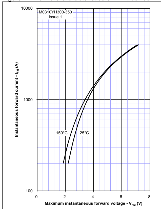
Figure 1 – Forward characteristics of Limit device
