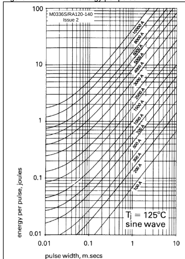
Figure 4 - Sine wave energy per pulse
