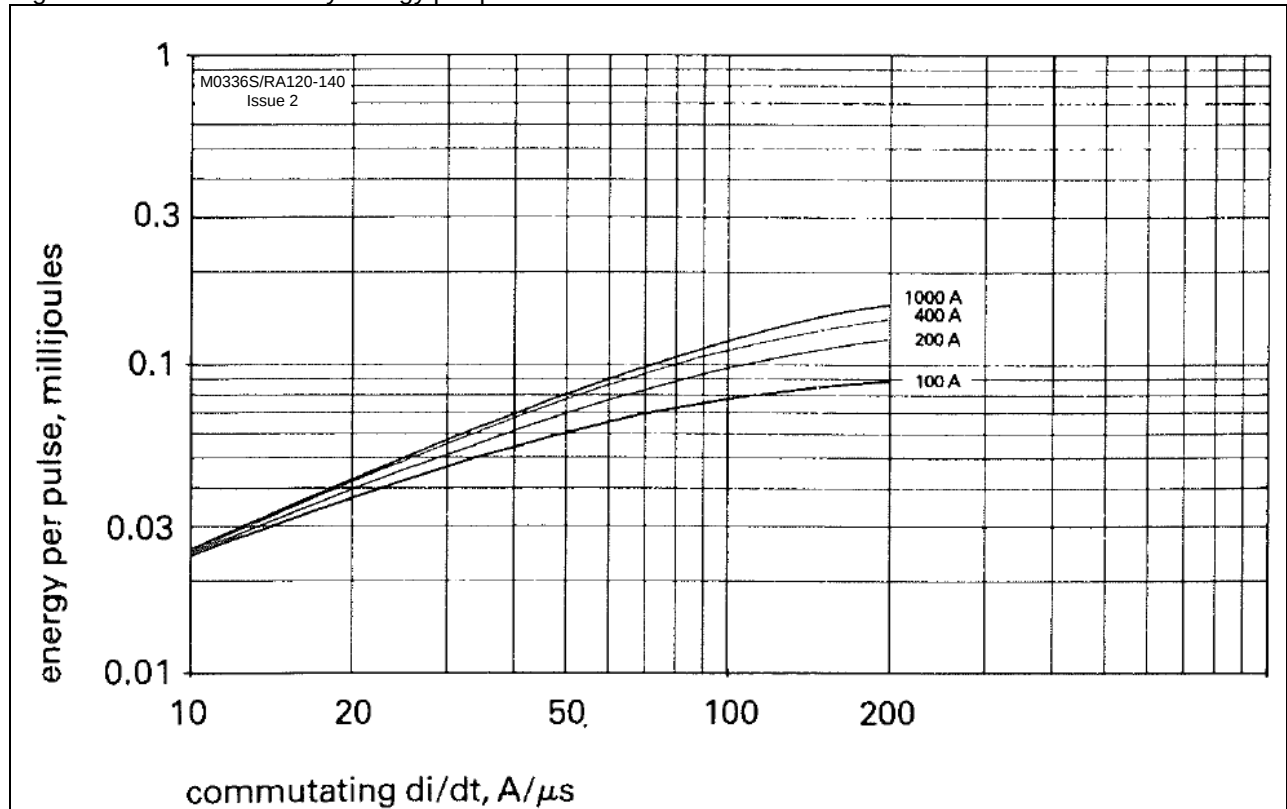
Figure 3 - Reverse recovery energy per pulse
