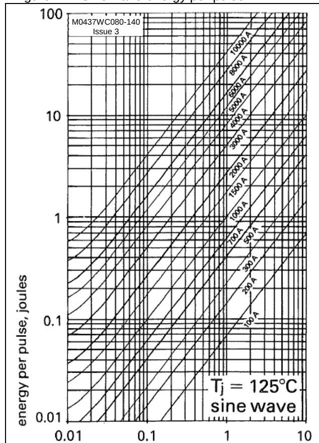
Figure 12 - Sine wave energy per pulse
