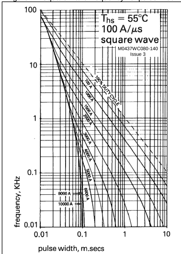
Figure 4 - Square wave frequency vs. pulse width
