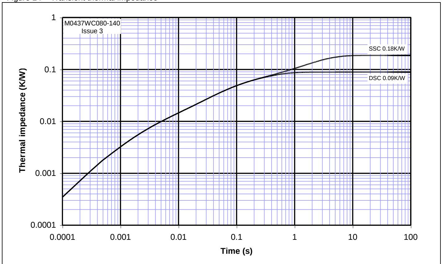
Figure 14 – Transient thermal impedance
