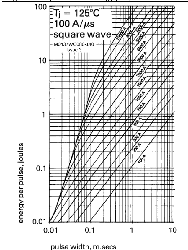
Figure 8 - Square wave energy per pulse
