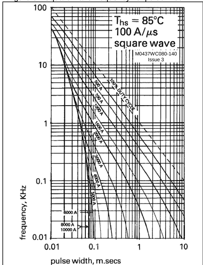
Figure 5 - Square wave frequency vs. pulse width
