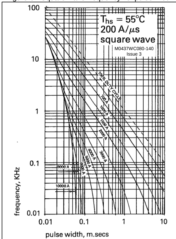
Figure 6 - Square wave frequency vs. pulse width
