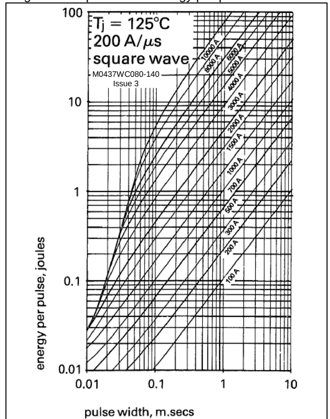
Figure 9 - Square wave energy per pulse
