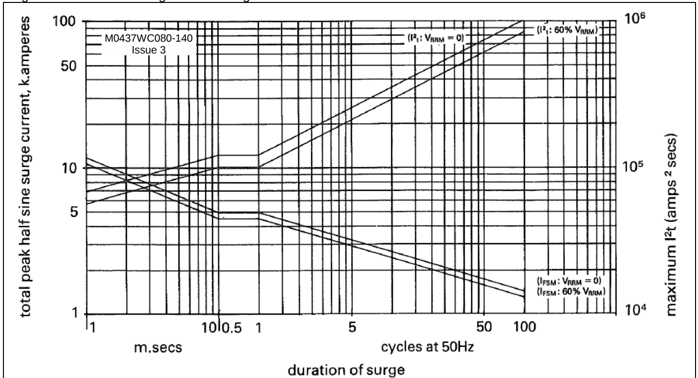
Figure 13 – Maximum surge and I^2t ratings
