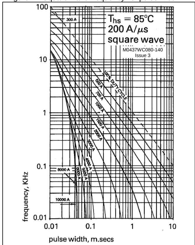
Figure 7 - Square wave frequency vs. pulse width
