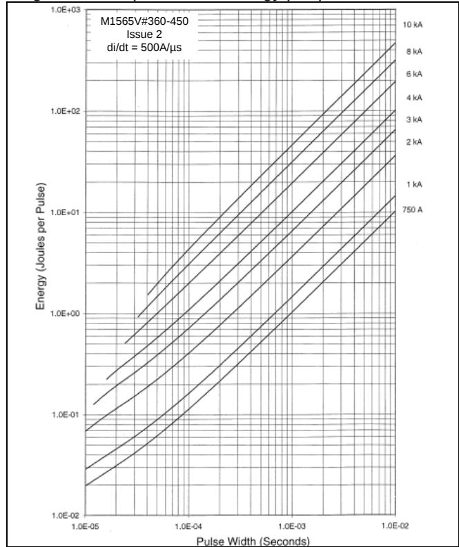
Figure 12 – Square wave energy per pulse
