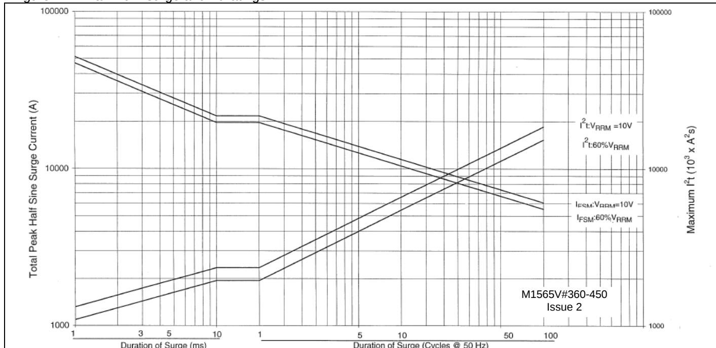
Figure 17 – Maximum surge and I^2t ratings
