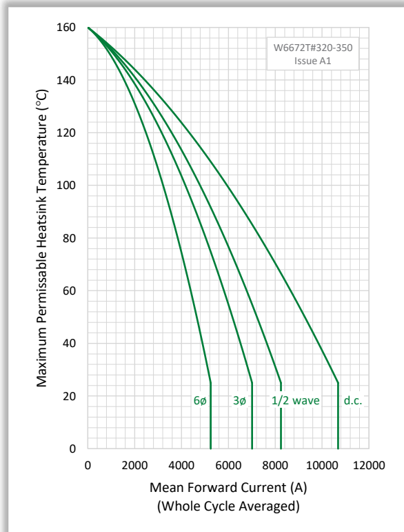
Figure 8. Forward Current vs. Heat Sink Temperature (Double Side Cooled)
